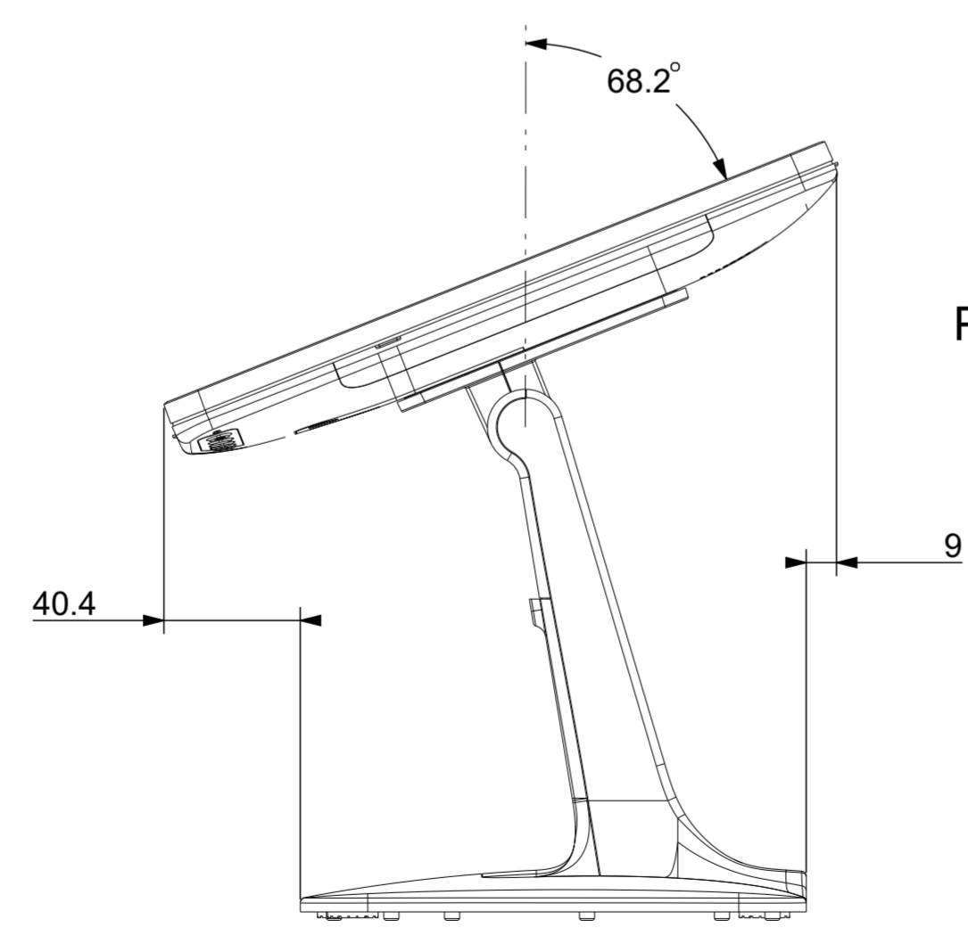
DISPLAY ANGLE RANGE IN HIGH POSITION
