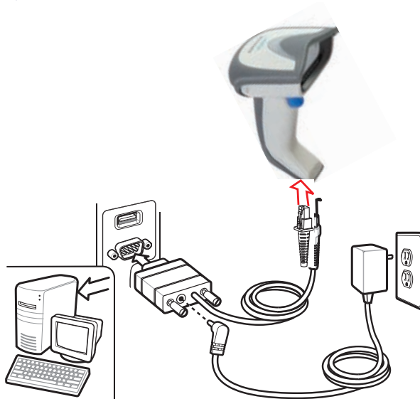
Figure 4. RS-232 Connection
